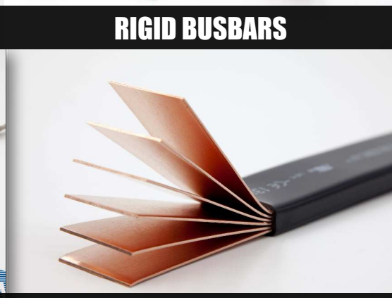
INSULATED FLEXIBLE BUSBAR
